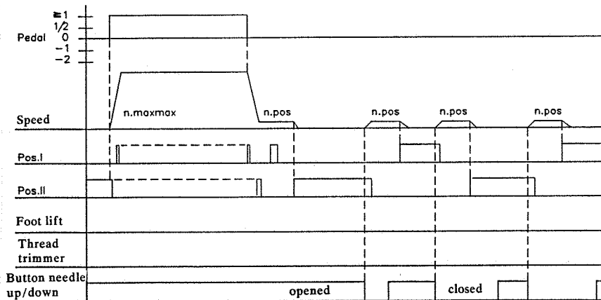
Function: needle up / down
