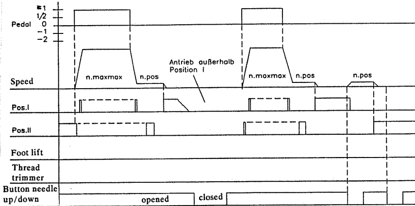
Function: needle up
