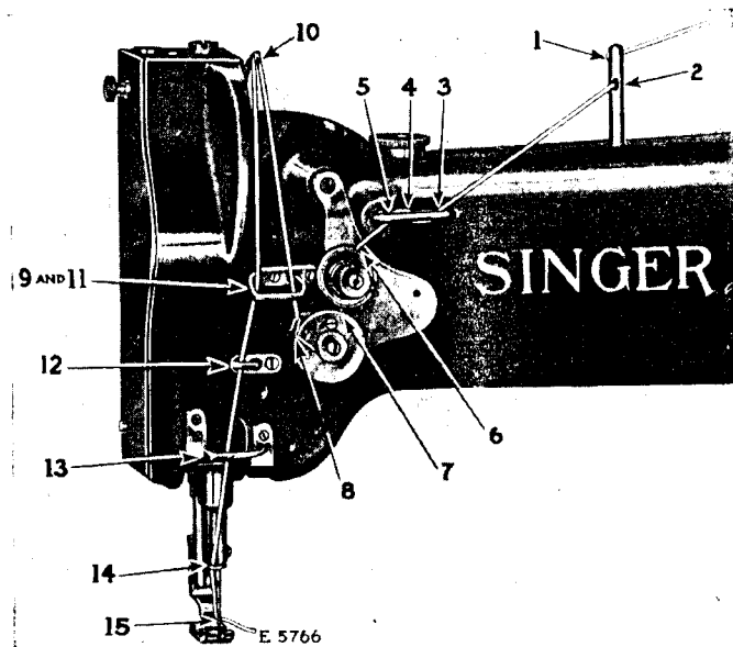
Fig. 7. Threading the Needle
