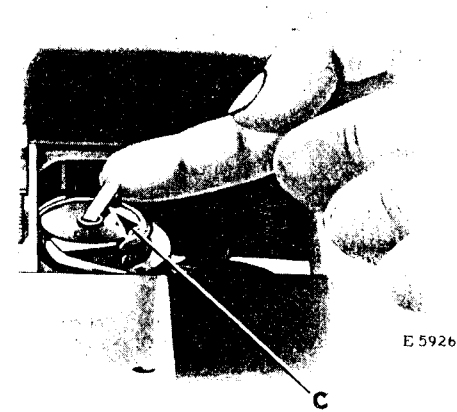
Fig. 3. Removing the Bobbin
