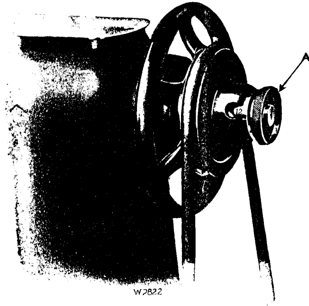
Fig. 11. Stitch Regulator
