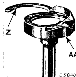
Fig. 18. Sewing Hook Removed from Machine, Showing Hook Washer
