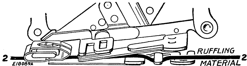
FIG. 62. CORRECT POSITION FOR MATERIAL TO BE RUFFLED
