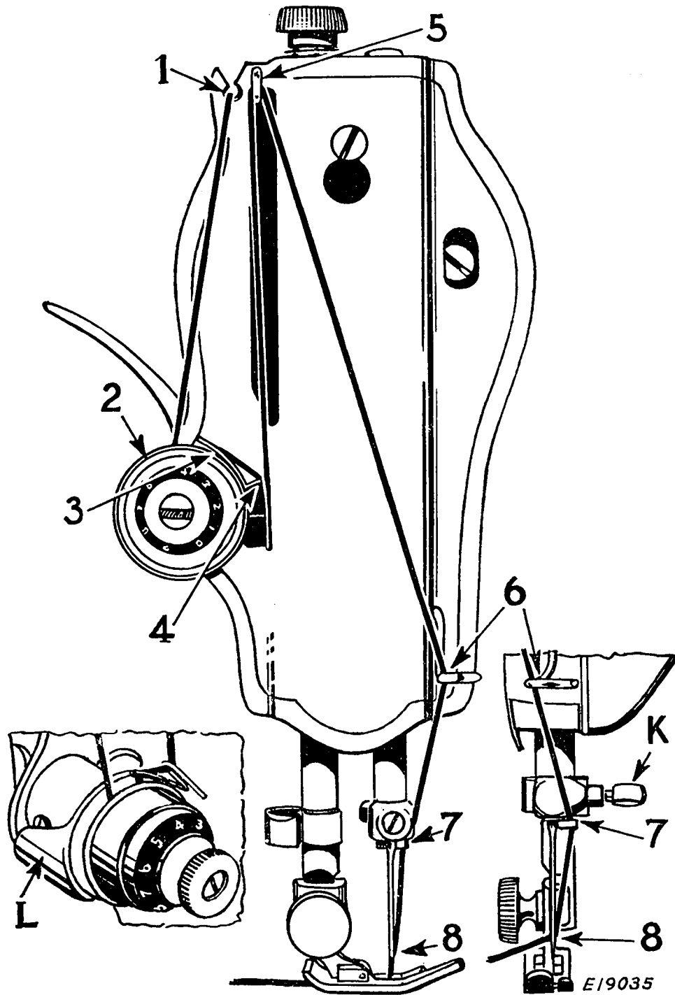
FIG. 6. UPPER THREADING
