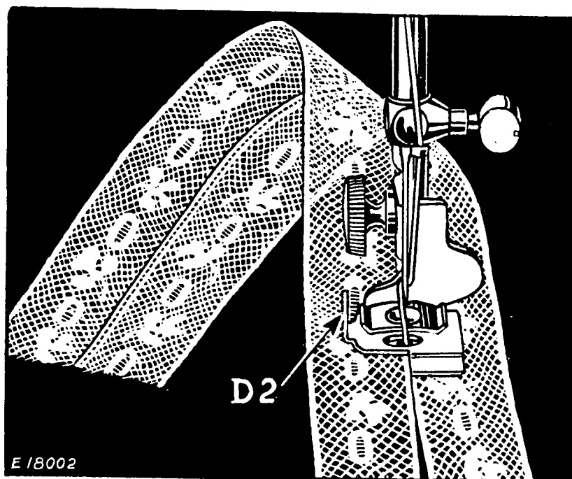
FIG. 52. SEWING LACE TOGETHER
