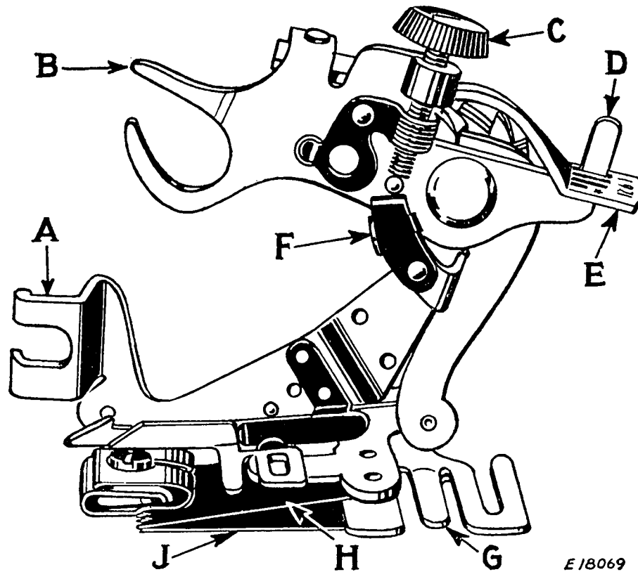
FIG. 60. PRINCIPAL PARTS OF THE RUFFLER
