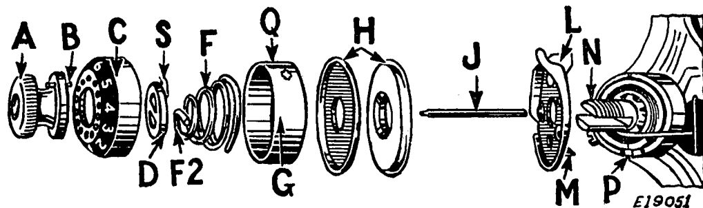
FIG. 22. NEEDLE THREAD TENSION DISASSEMBLED
