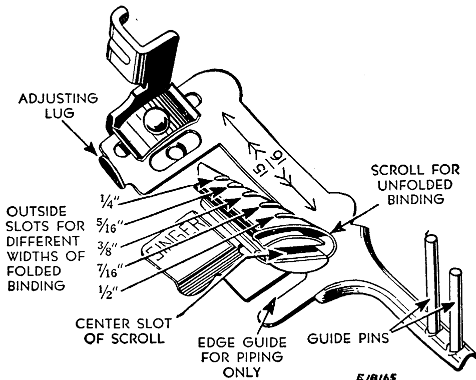
FIG. 44. MULTIPLE SLOTTED BINDER 160359
