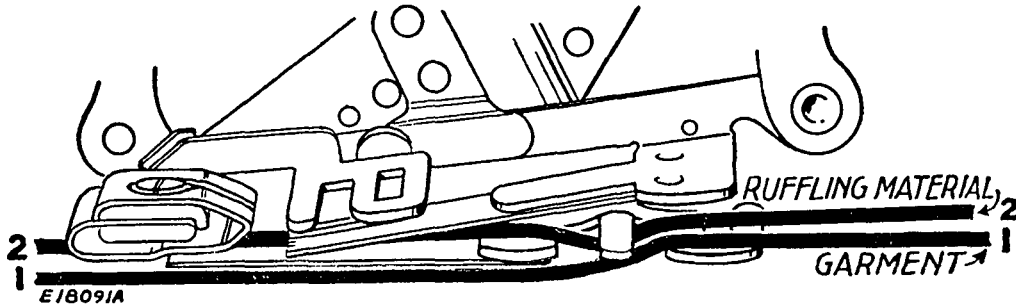
FIG. 63. CORRECT POSITIONS FOR THE MATERIALS
