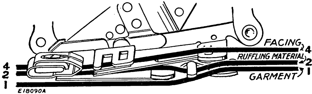
FIG. 65. CORRECT POSITIONS FOR THE MATERIALS
