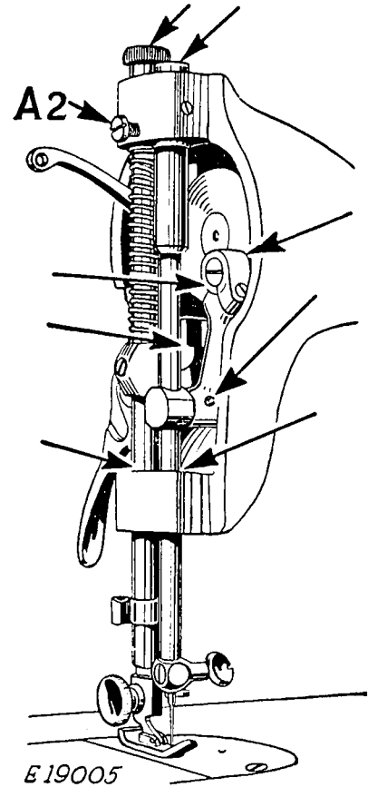
FIG. 27. END VIEW SHOWING OILING POINTS
