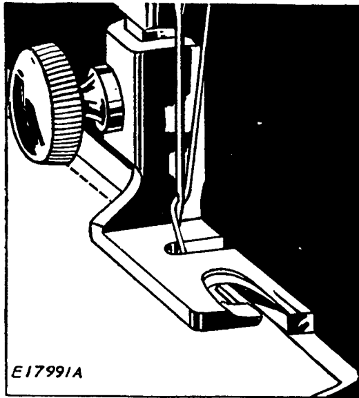
FIG. 39. MAKING A FELLED SEAM (FIRST OPERATION)
