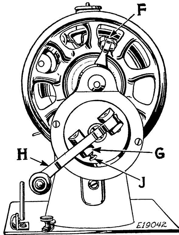
FIG. 4. END VIEW OF MACHINE 15-89 SHOWING HAND DRIVING ATTACHMENT
