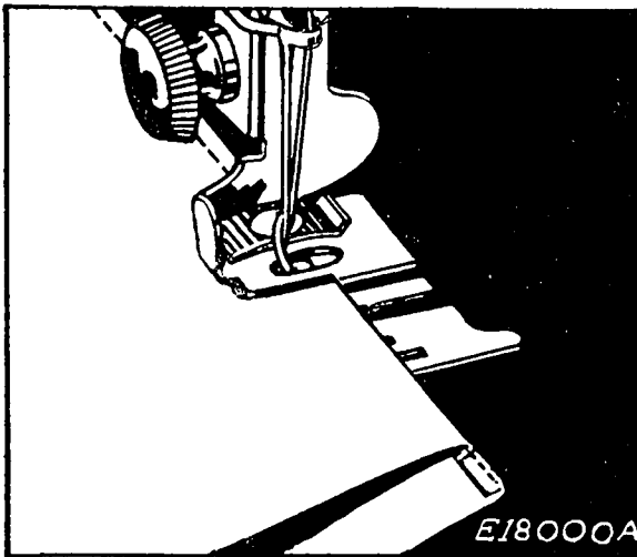
FIG. 57. MAKING A FRENCH SEAM (SECOND OPERATION)
