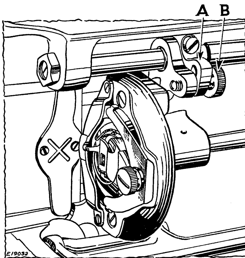
FIG. 32. ADJUSTMENT FOR DARNING OR EMBROIDERING
