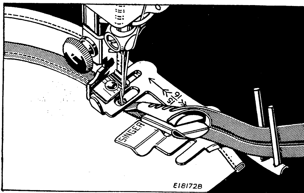
FIG. 50. APPLYING A FRENCH FOLD
