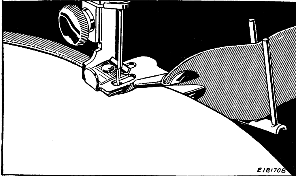
FIG. 49. BINDING AN OUTSIDE CURVE
