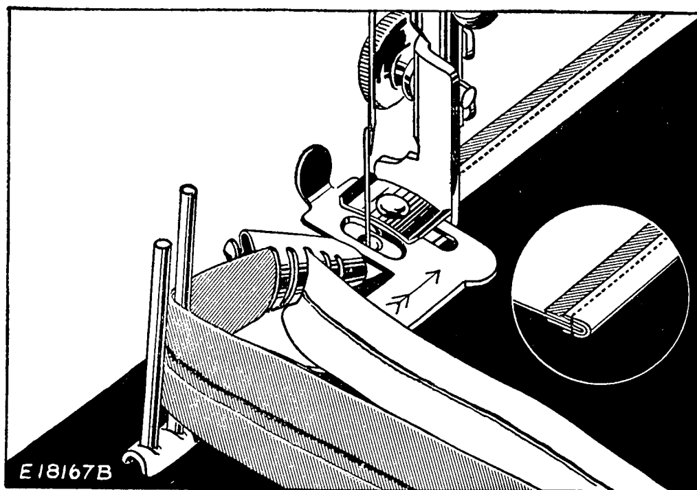
FIG. 48. PIPING AND BINDING IN ONE OPERATION
