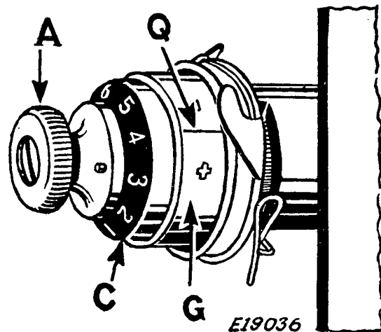
FIG. 21. NEEDLE THREAD TENSION
