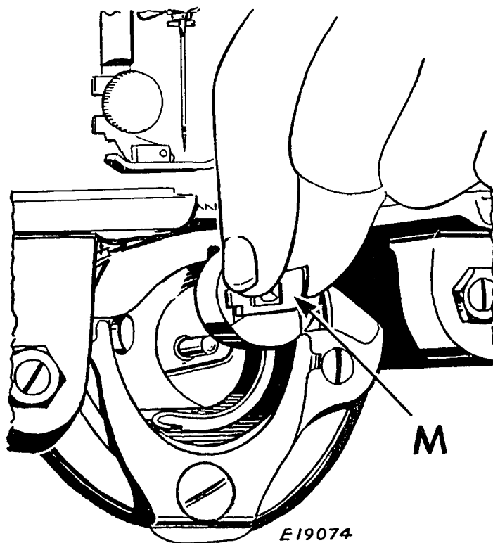
FIG. 7. REMOVING THE BOBBIN CASE
