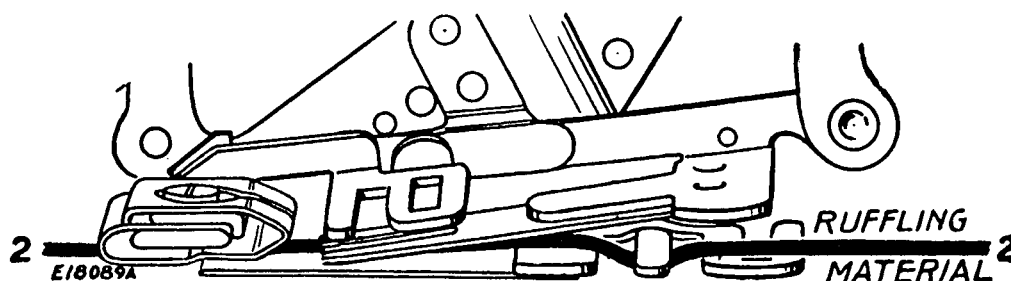
FIG. 70. CORRECT POSITION FOR THE MATERIAL
