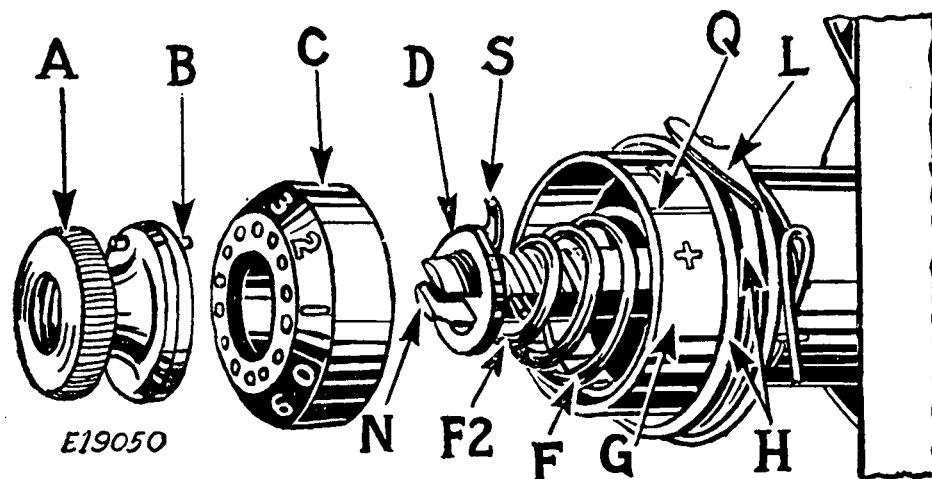
FIG. 23. REASSEMBLING AND REPLACING THE TENSION
