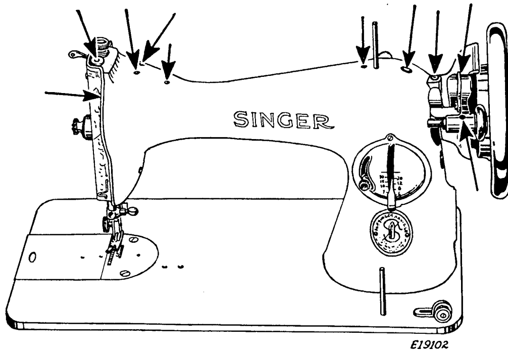
FIG. 25. FRONT VIEW, SHOWING OILING POINTS
