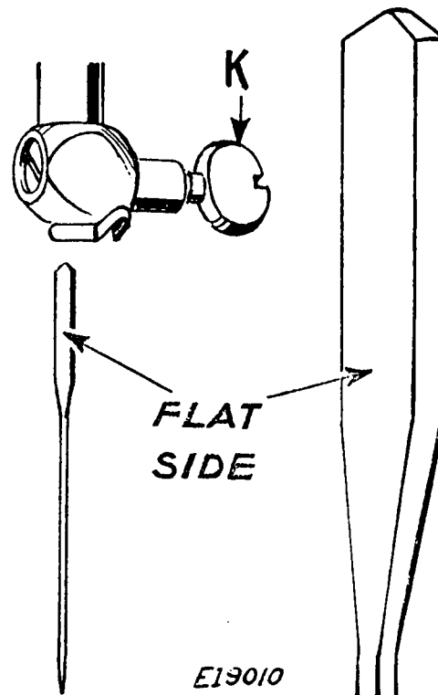
FIG. 5. SETTING THE NEEDLE
