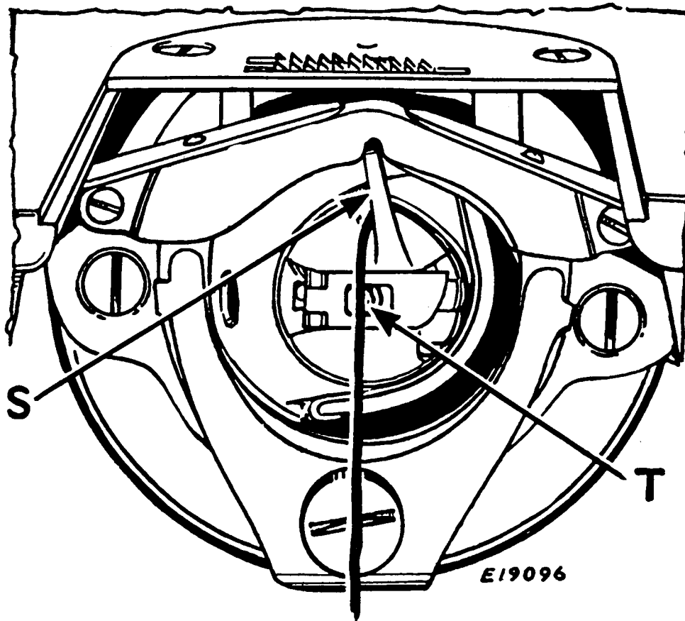
FIG. 13. BOBBIN CASE THREADED AND REPLACED
