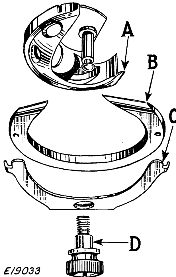
FIG. 31. SHUTTLE AND PARTS REMOVED FROM MACHINE
