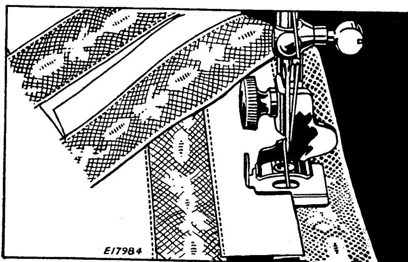
FIG. 53. SETTING IN LACE INSERTION
