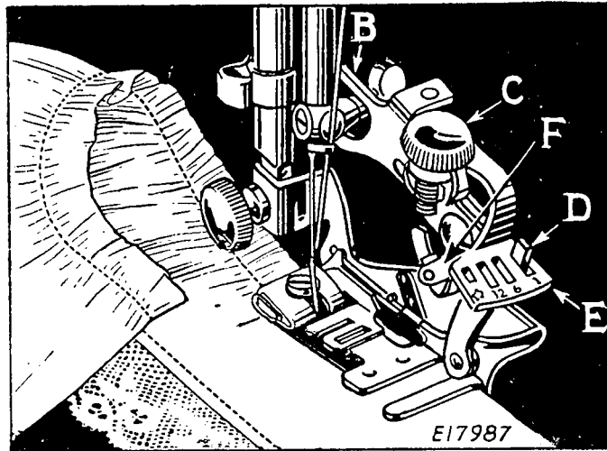
FIG. 61. GATHERING WITH THE RUFFLER
