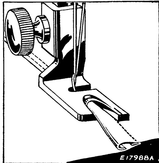
FIG. 40. MAKING A FELLED SEAM (SECOND OPERATION)
