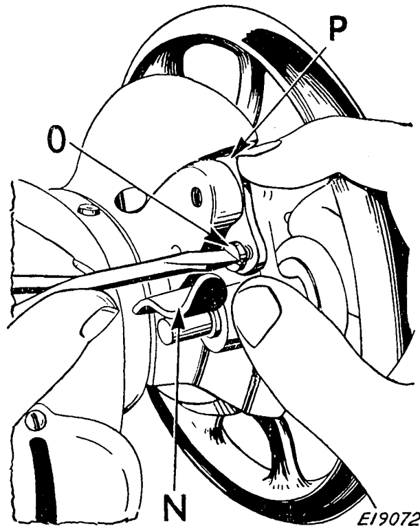
FIG. 9. ADJUSTMENT OF BOBBIN WINDER
