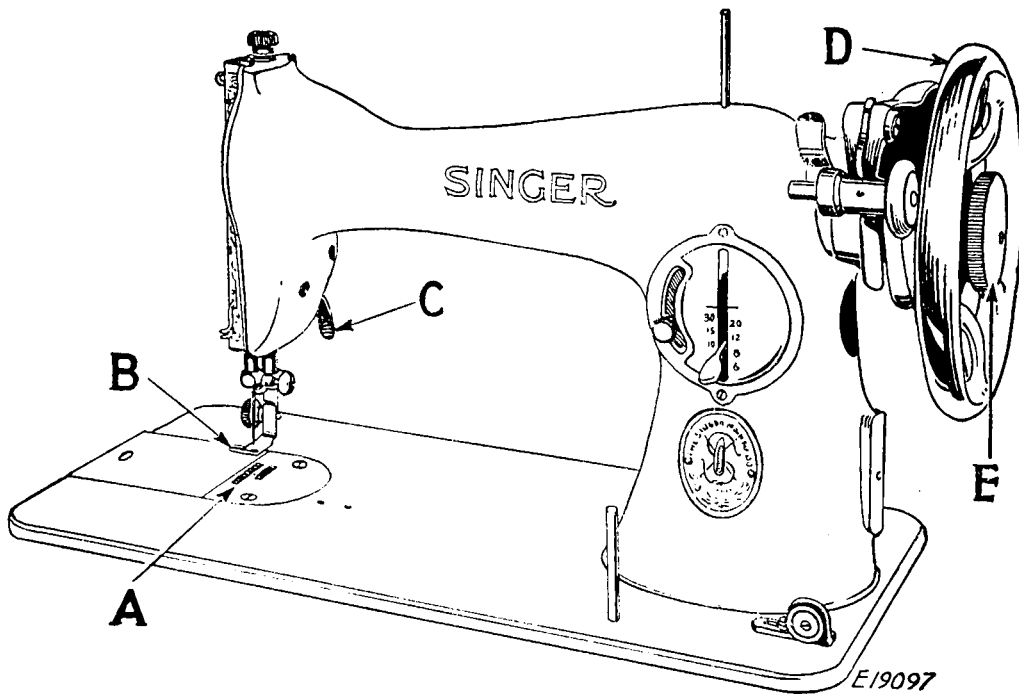
FIG. 3. FRONT VIEW OF THE MACHINE
