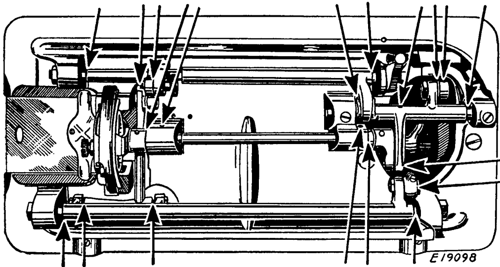
FIG. 29. OILING POINTS IN BASE OF MACHINE
