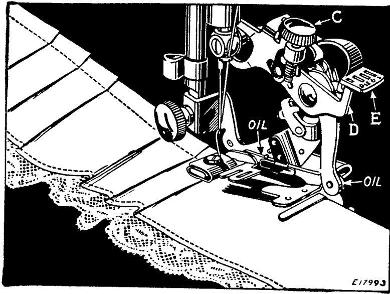
FIG. 71. GROUP PLAITING WITH THE RUFFLER
