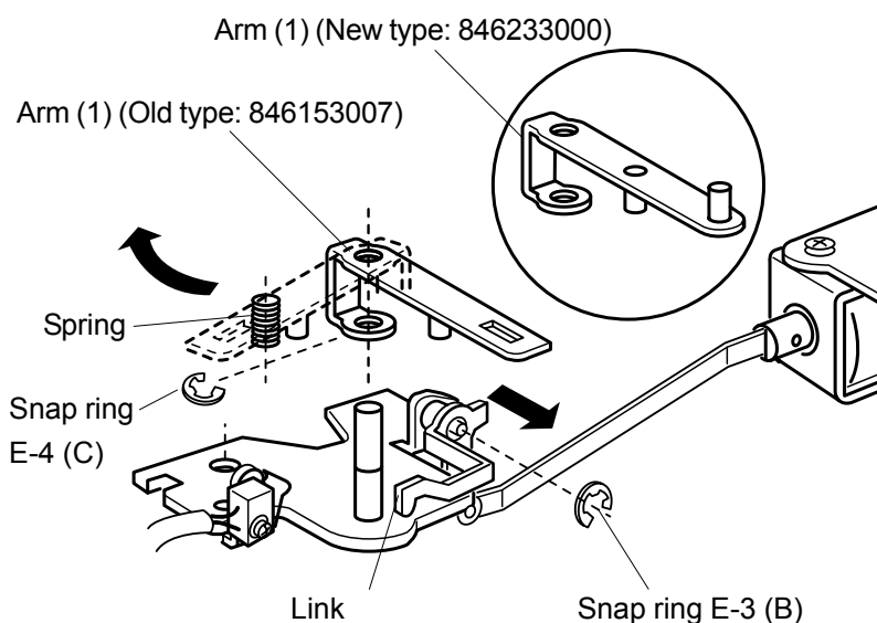
Thread cutter unit (New type)
