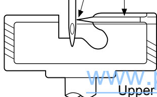
Hook race
