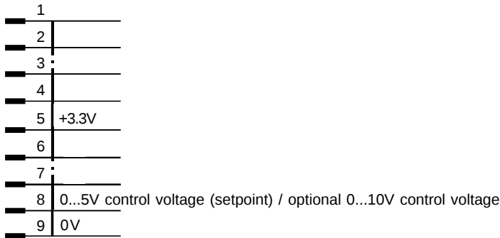
Contact assignment of the connecting plug (X3) on the SCU2 (Fig. 7.13)
