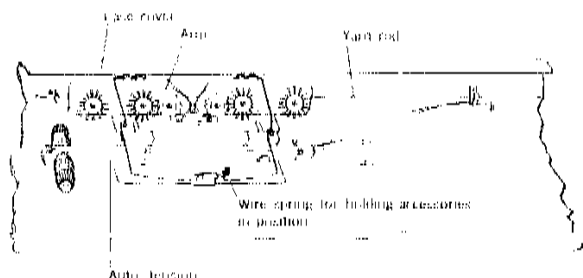
(8) Release the wire spring which holds the accessories in position inside the case cover and remove the carriage arm.
