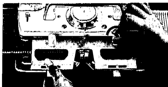
(9) Loosen the nuts on the carriage arm and push in the arm as far as it goes and tighten the nuts firmly.
