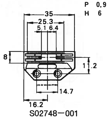
送り歯 Feed Dog
