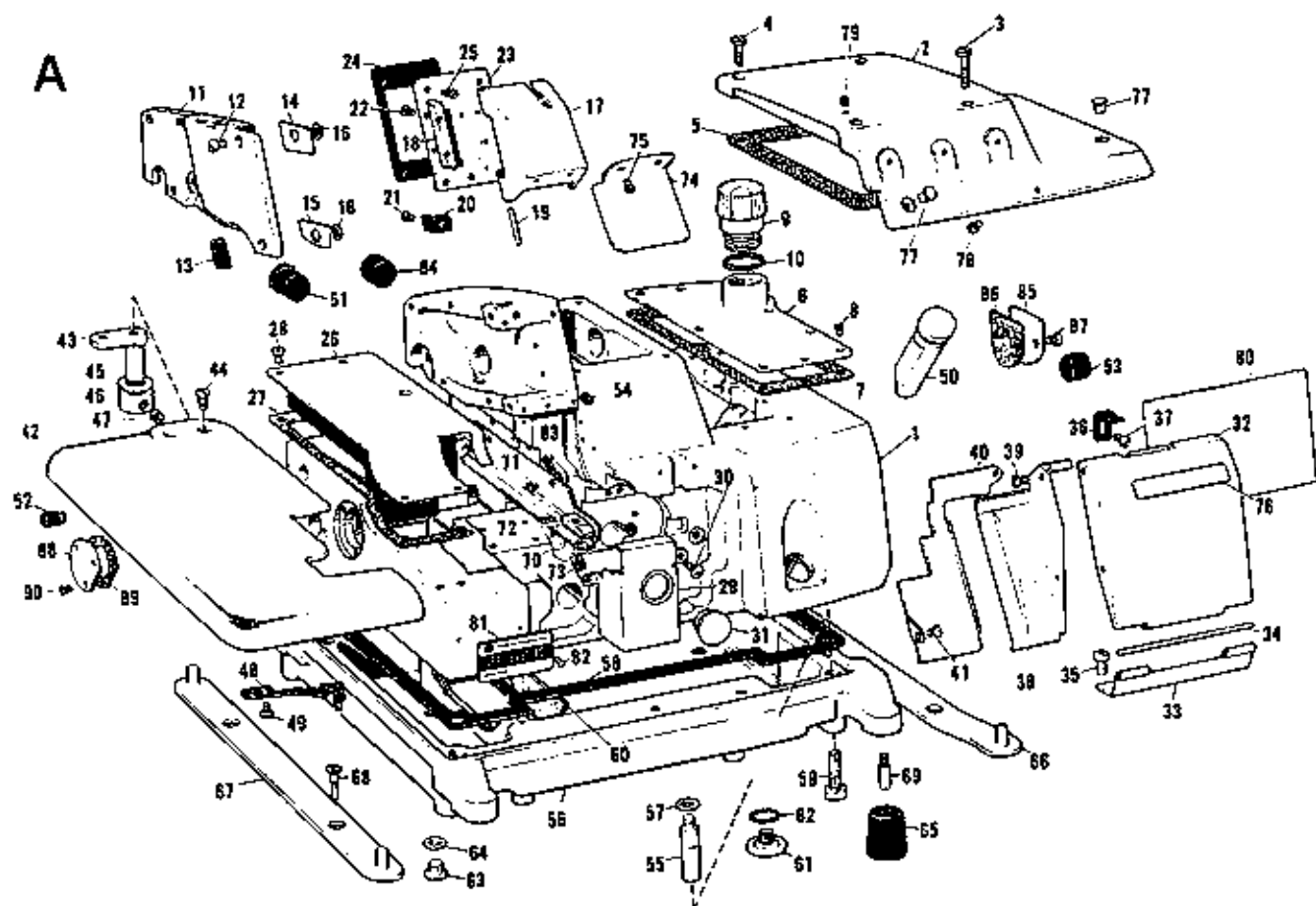
PARTS LIST for EF4-B957-1C
