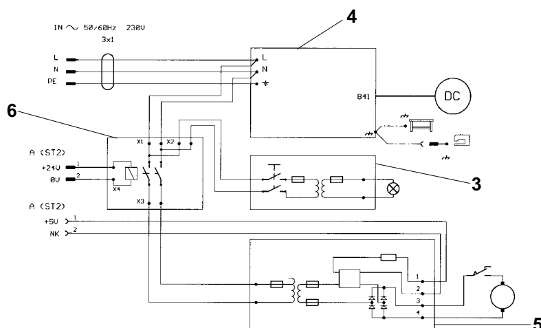
Circuit layout
